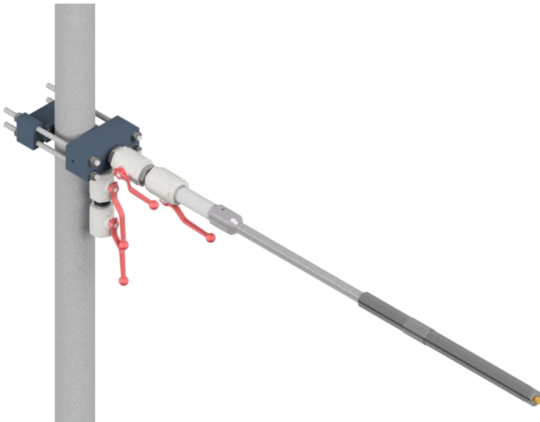
Hot tap setup with double valves
